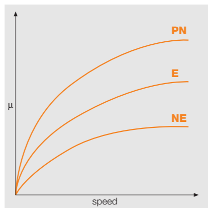
Friction diagramm
